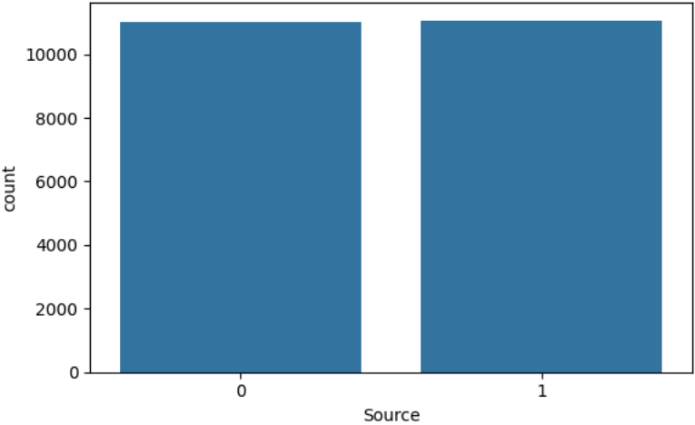
Count Plot: Source (Industry vs Commodity)
